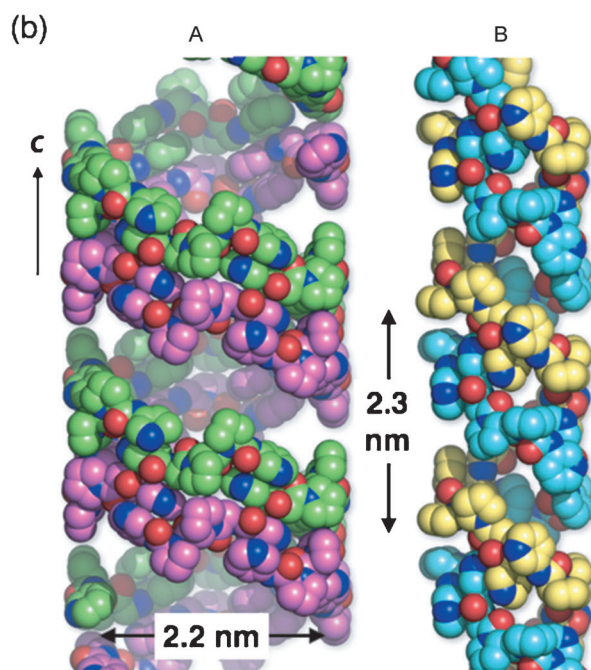
Figure 3. Nanochannel structure in [(\text{AgBF}_4) \cdot \mathbf{1}]_n . a) Top view: within the whole framework (blue stick representation), larger nanochannel A is highlighted in green/magenta space-filling representation and smaller nanochannel B in cyan/yellow. b) Side view: space-filling representation of nanochannel frameworks A and B. One pseudo-strand (green or magenta) is formed not by chemical bonds but by connection through \pi -stacking of the py groups. Two such pseudo-strands form a left-handed duplex-like structure (22.8 Å pitch). All solvents and hydrogen atoms have been omitted for clarity.
